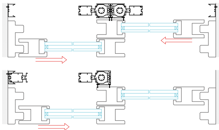
Detached "C" profile installation mode
